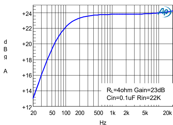
Frequency Response
